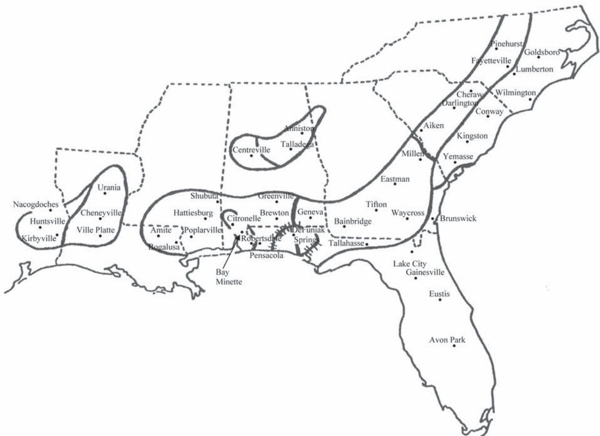
Figure 1—The climatic zones of the longleaf pine region.
